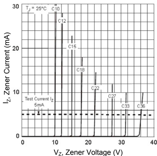
Figure 3. Typical Zener Breakdown Characteristics
