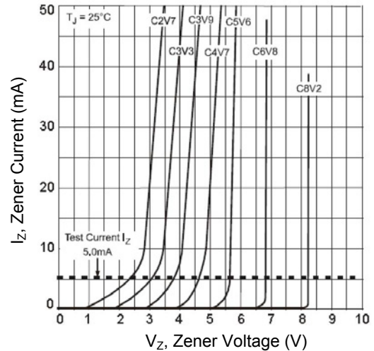
Figure 2. Typical Zener Breakdown Characteristics
