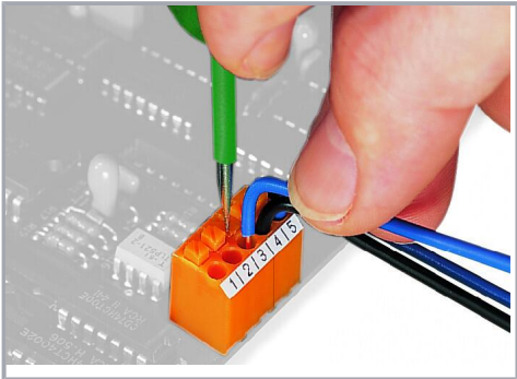
Removing a conductor via push-button.
