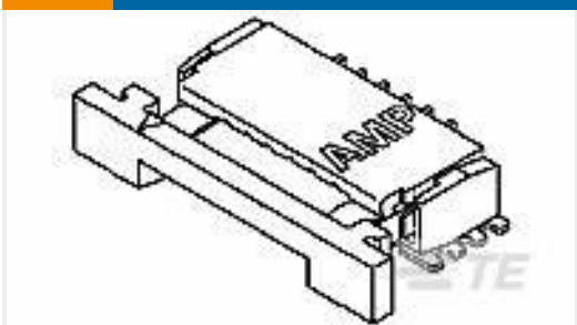
TE Part # 2-84952-0 1MM FPC HORZ.BTTM CONT.ASS.20P
