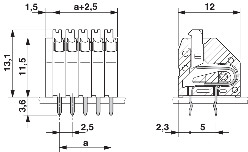
Dimensional drawing
