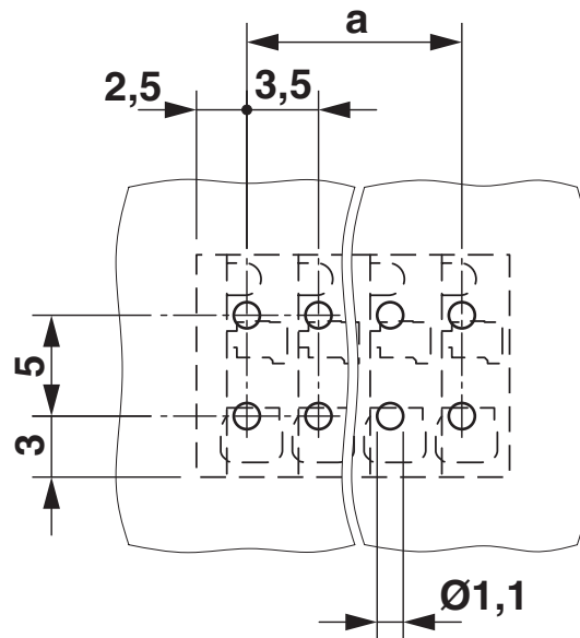
Dimensional drawing
