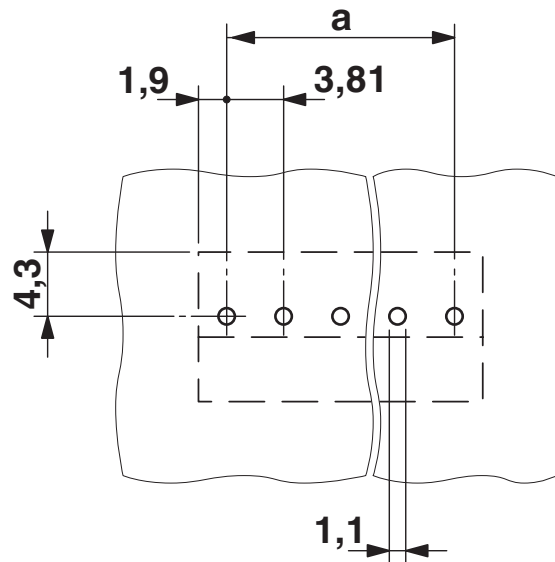
Dimensional drawing
