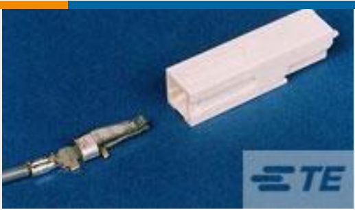
TE Part # 556137-2 HSG,AMPINERGY WTW,1 POS, BLACK
