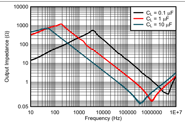
Figure 6-32. Output Impedance
