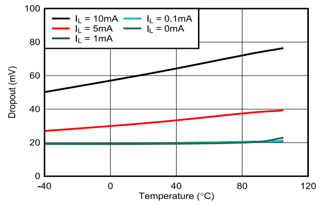
Figure 6-34. Dropout Voltage vs Free-Air Temperature
