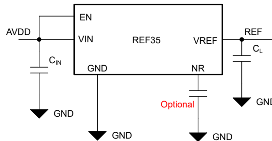
Figure 8-1. Basic Connections
