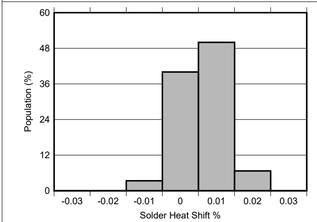
Figure 6-35. Solder Heat Shift Distribution
