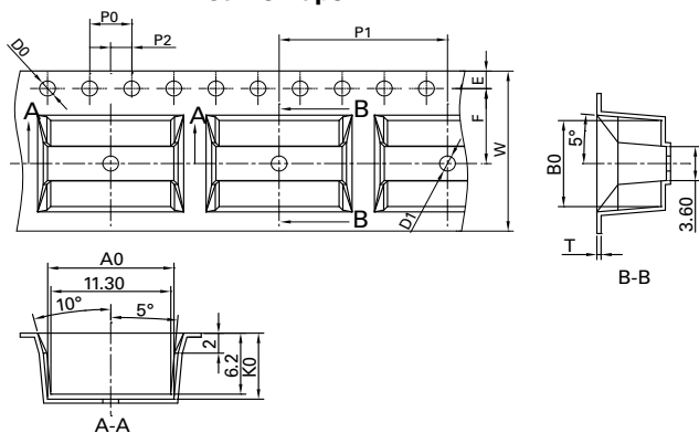
Carrier Tape
