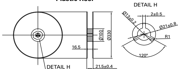
Plastic Reel
