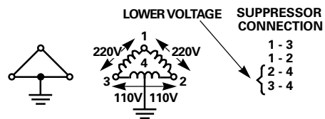
FIGURE 25D. 3 PHASE 220V
