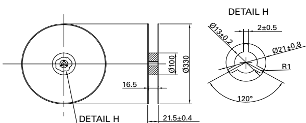
Plastic Reel
