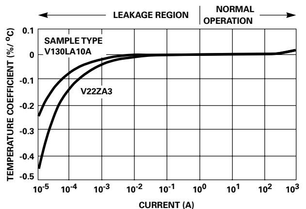
FIGURE 14. RELATION OF TEMPERATURE COEFFICIENT dV/dT TO VARISTOR CURRENT
