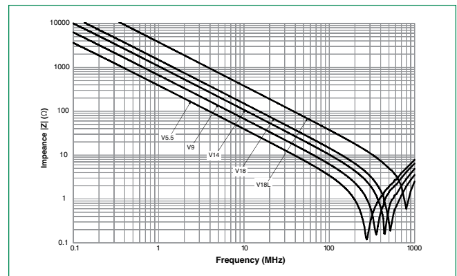
Fig. 4 Impedance vs Frequency, 1206 Size
