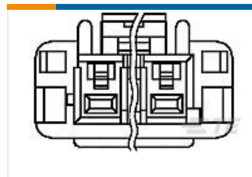
TE Part #1376390-1 5MM POWER KEY 4P PLUG HSG NUT
