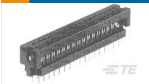
TE Part # 1658525-2 622-3453LF, PCB IDC, LEAD FREE
