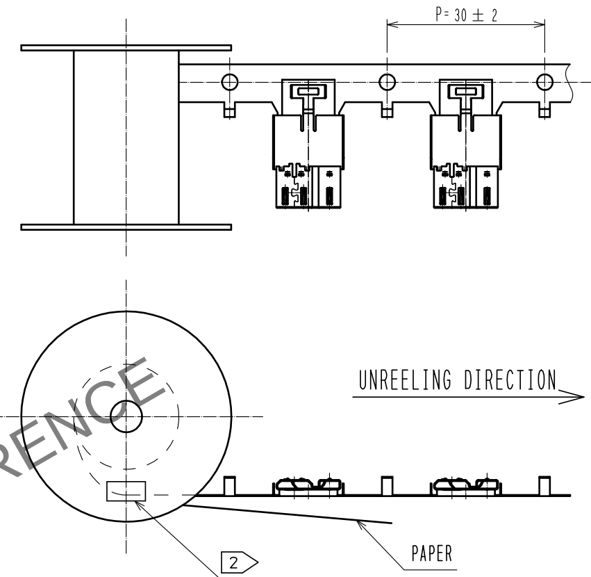
1 Fig-1 DRAWING FOR PACKING (FREE)
