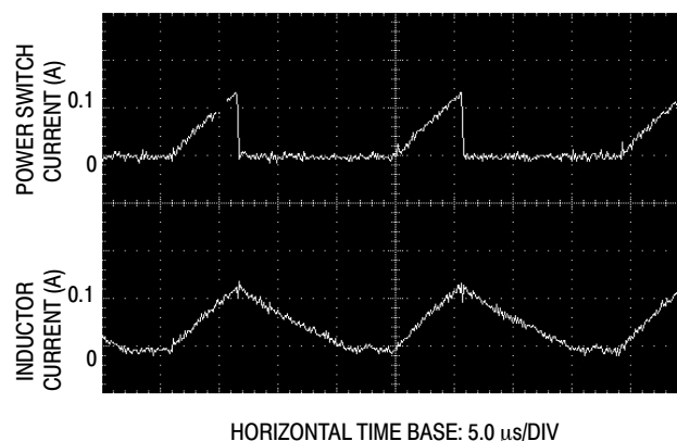
Figure 23. Discontinuous Mode Switching Current Waveforms
