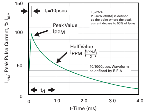
Figure 4 - Pulse Waveform
