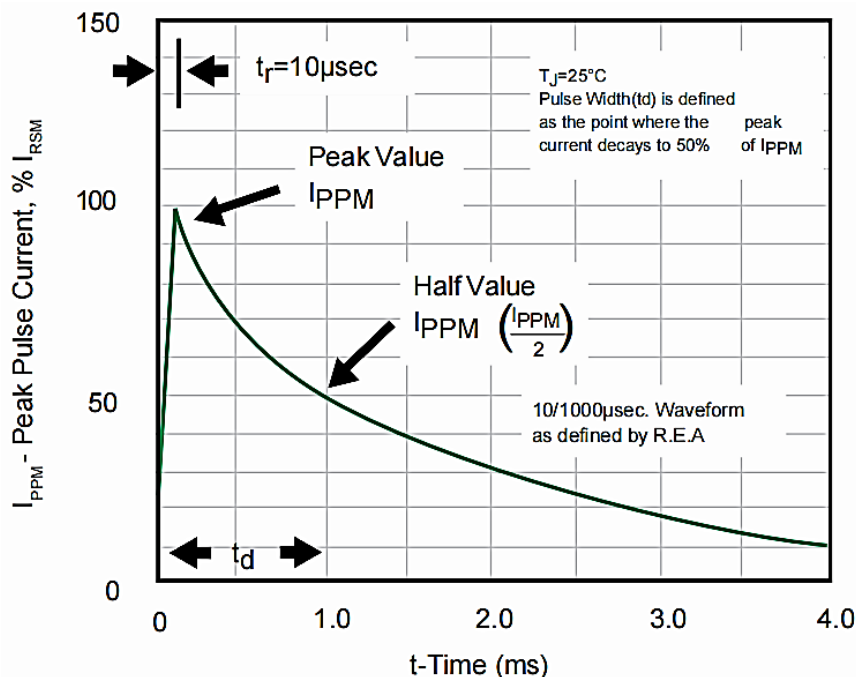
Figure 3. Pulse Waveform
