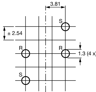
Hole pattern
