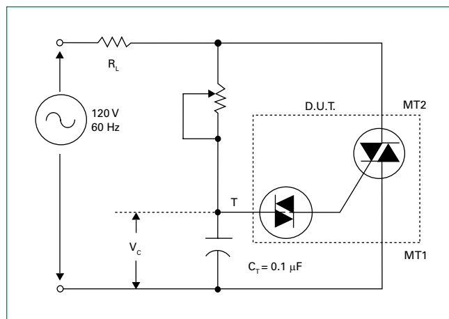
Figure 7: Test Circuit
