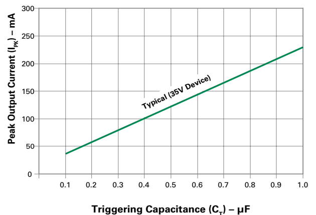
Figure 11: Peak Output Current vs Triggering Capacitance (Per Figure 9)
