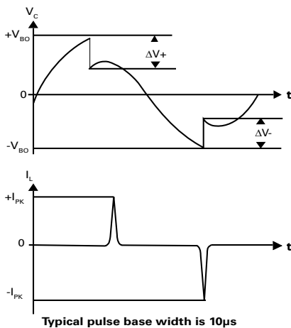
Figure 10: Test Circuit Waveform
