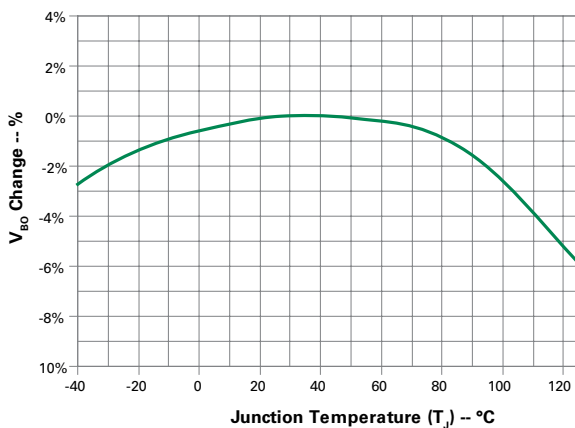
Figure 8: DIAC V_{BO} Change vs. Junction Temperature
