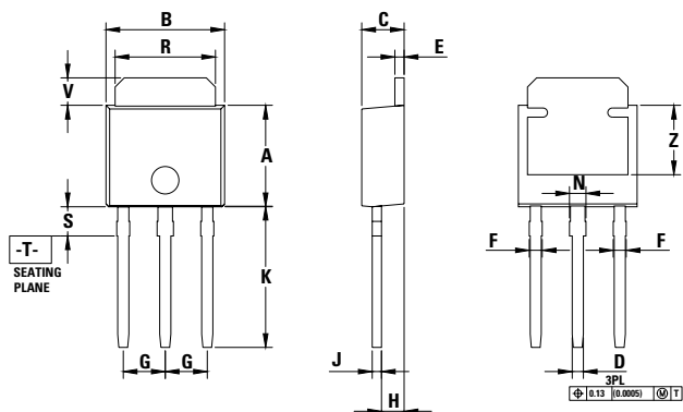
DDAK-3 Case 369D-01 Issue B T0251-3L POD
