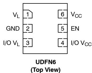
Figure 6. Pin Assignments
