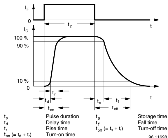
Fig. 4 - Switching Times
