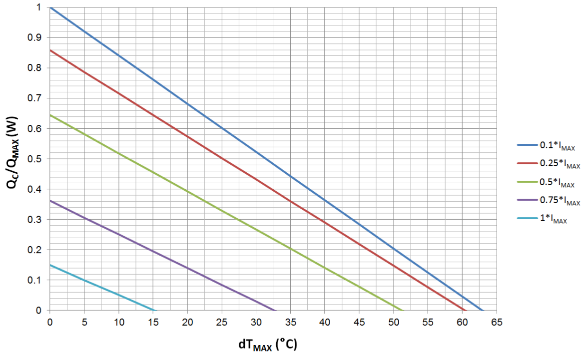
Figure 6. Q_c/Q_{MAX} vs. dT_{MAX}
