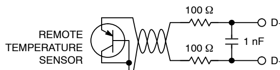
Figure 23. Filter Between Remote Sensor and ADT7467
