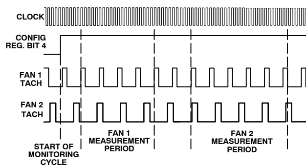
Figure 24. Fan Speed Measurement
