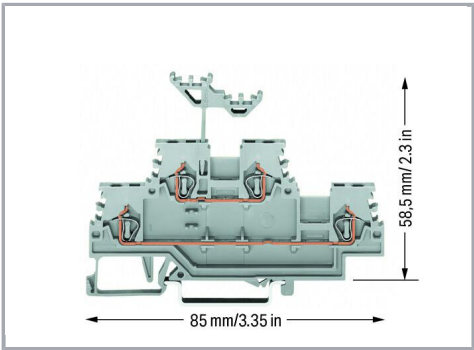
Double-deck marker carrier (height including marker carrier)
