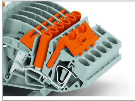
Jumper with safety lid Longitudinal switching disconnect terminal blocks with inserted jumper, including safety lid
