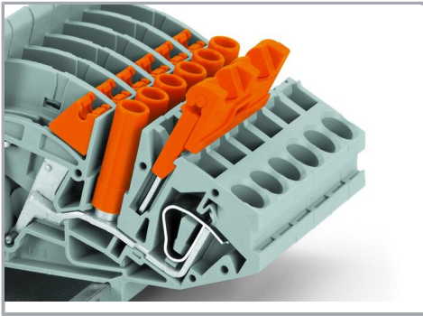
Jumper with safety lid Jumper in pre-locked position
