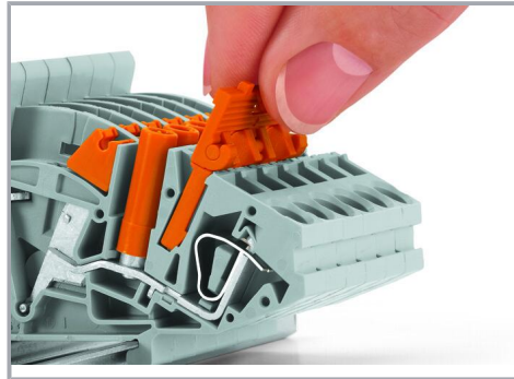
Jumper with safety lid Removing a jumper via safety lid.
