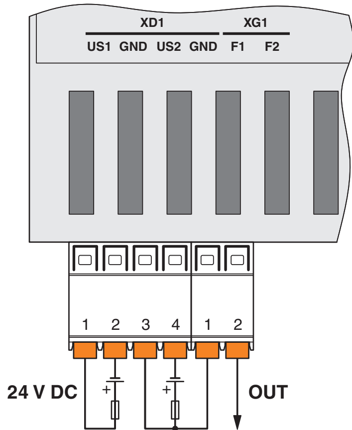
Connection diagram
