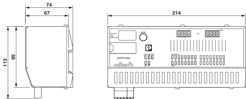
Dimensional drawing
