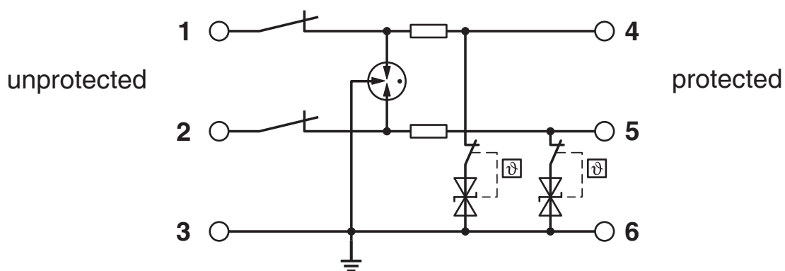
Circuit diagram
