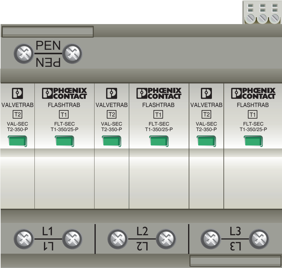
Product drawing
