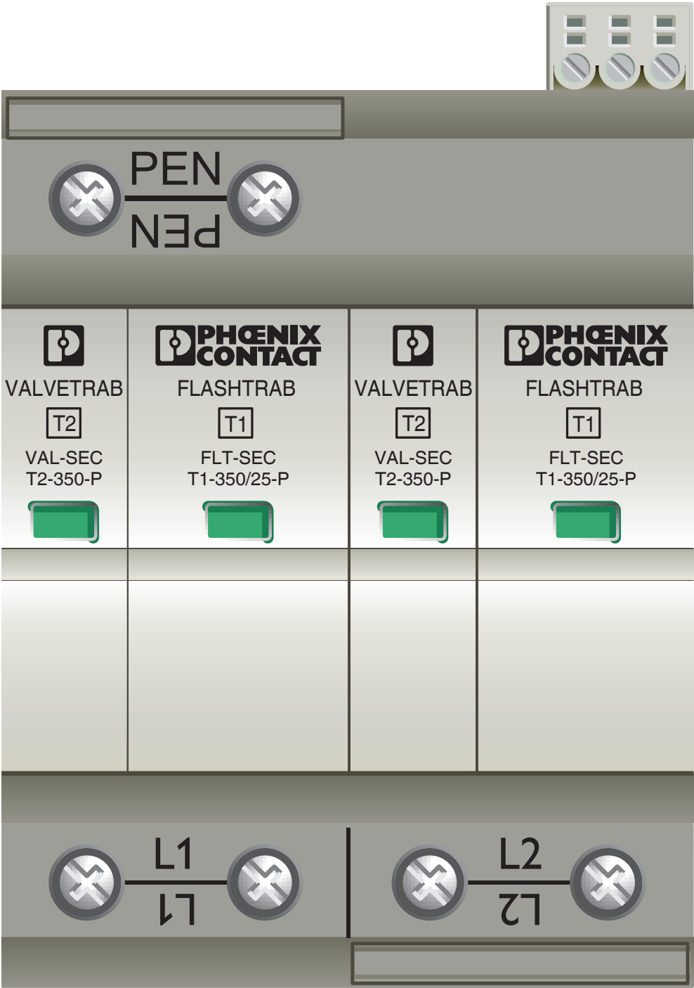
Product drawing
