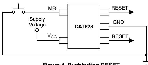
Figure 4. Pushbutton RESET
