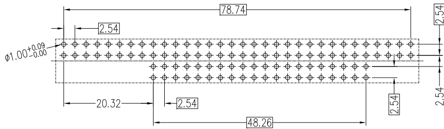
Recommended P.C.B Layout for 52pins (Top Side) (PCB BOARD TOLERANCE±0.05)
