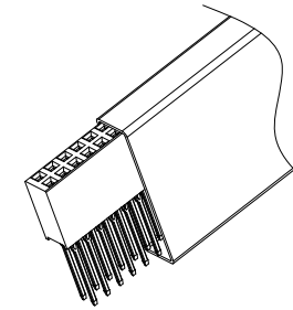
3D View for 32pins & 20pins After packing
