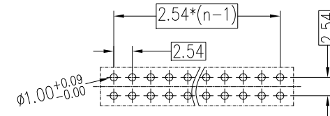
Recommended P.C.B Layout for 32pins & 20pins (Top Side) (PCB BOARD TOLERANCE±0.05)
