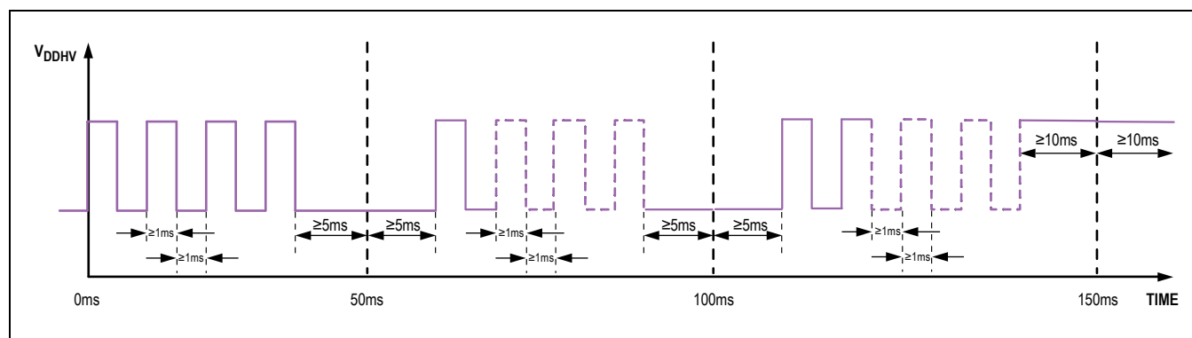
Figure 7. Power Line Communication Activation Timing
