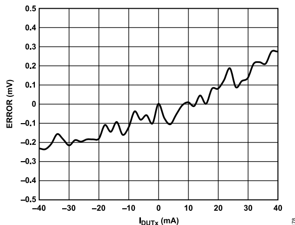
Figure 78. PPMU Force Voltage Compliance Error, Range A, FV = -1.0 V vs. Output Current, Internal Sense
