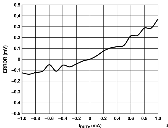
Figure 80. PPMU Force Voltage Compliance Error, Range B, FV = -1.5 V vs. Output Current ( I_{DUTx} ), Internal Sense
