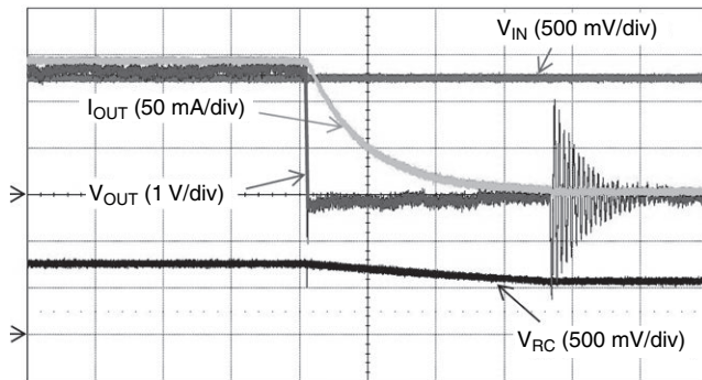
5 \mu s/div V_{IN} = 2.8 V, R_{LOAD} = 18 \Omega , L_{LOAD} = 80 \mu H Inductive Discharge OUT1 to OUT2
