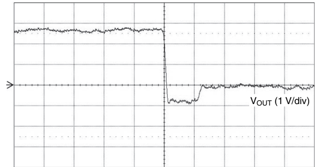
50 ns/div V_{IN} = 2.8 V, R_{LOAD} = 18 \Omega , L_{LOAD} = 80 \mu H Falling Edge T_{BBM}
