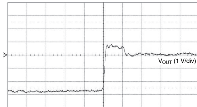
50 ns/div V_{IN} = 2.8 V, R_{LOAD} = 18 \Omega , L_{LOAD} = 80 \mu H Rising Edge T_{BBM}
