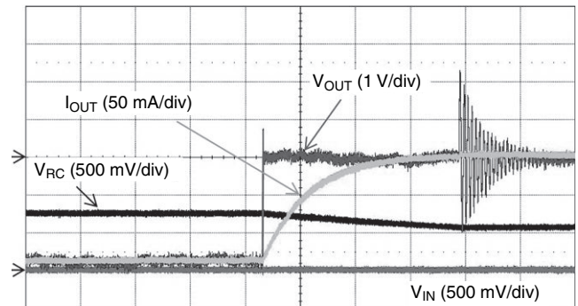
5 \mu s/div V_{IN} = 2.8 V, R_{LOAD} = 18 \Omega , L_{LOAD} = 80 \mu H Inductive Discharge OUT2 to OUT1
