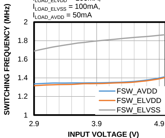
Switching Frequency vs. V_{IN}
