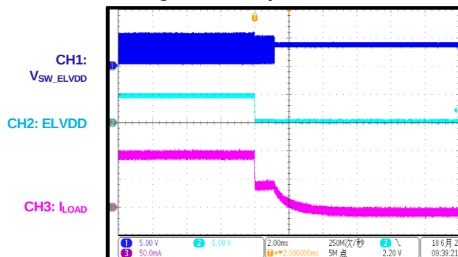
ELVDD Short to GND Protection during Normal Operation
