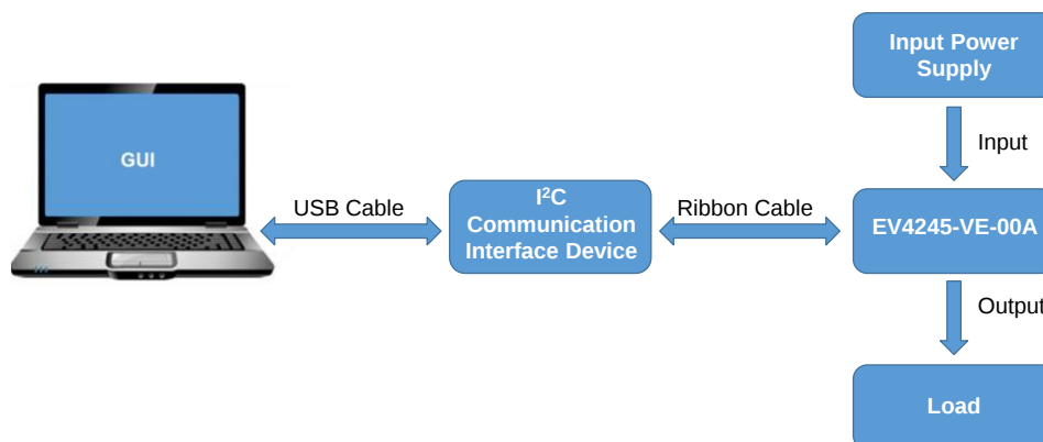
Figure 1: EVKT-MP4245 Evaluation Kit Set-Up
