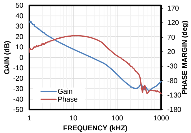
Bode Plot
