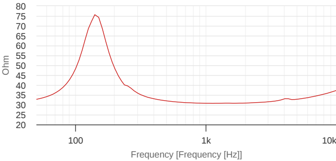
Impedance
