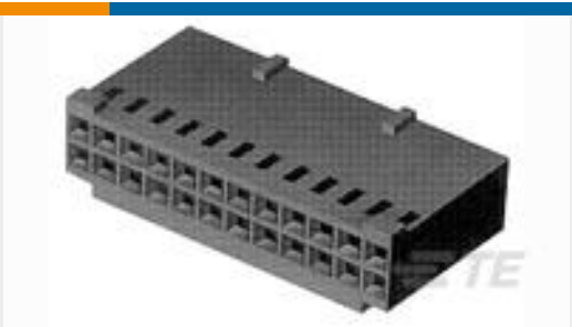
TE Part #87977-2 08 MODIV HSG DR MRKD .100 POL
