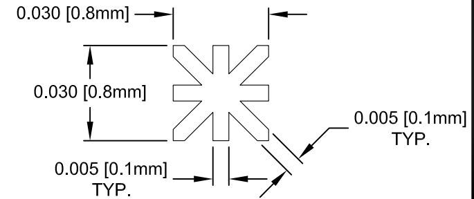
DETAIL B SCALE 5:1
