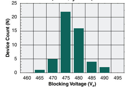
Typical Blocking Voltage Distribution (N=50, I_F=2\text{mA} )
