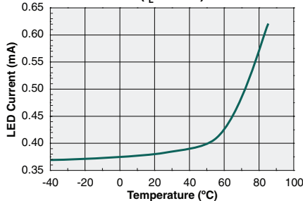
LED Current to Operate vs. Temperature ( I_L=75\text{mA} )
