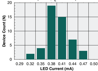
Typical LED Current to Operate (N=50, I_L=100\text{mA} )
