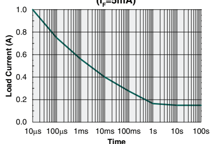
Energy Rating Curve, Single Pole ( I_F=5\text{mA} )
