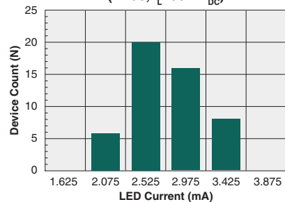
Typical I_F for Switch Operation (N=50, I_L=50\text{mA}_{DC} )
