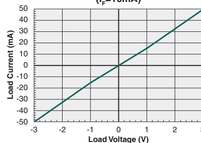
Typical Load Current vs. Load Voltage ( I_F=10\text{mA} )
