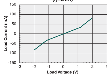
Typical Load Current vs. Load Voltage ( I_F=8\text{mA} )
