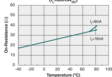
Typical On-Resistance vs. Temperature ( I_L=85\text{mA}_{\text{DC}} )
