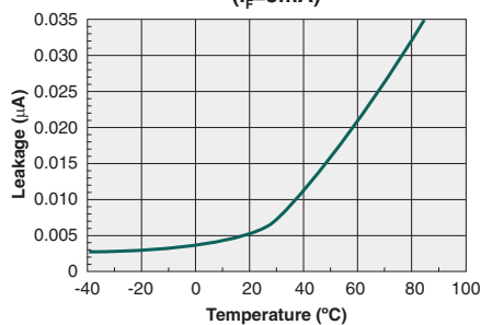
Form-B Typical Leakage vs. Temperature Measured across Pins 7&8 ( I_F=5\text{mA} )
