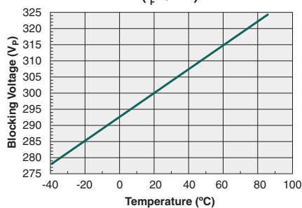
Form-B Typical Blocking Voltage vs. Temperature ( I_F=5\text{mA} )
