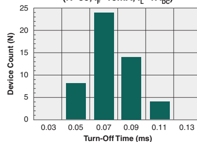
Typical Turn-Off Time (N=50, I_F=10\text{mA} , I_L=1A_{DC} )
