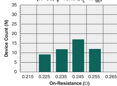
Typical On-Resistance Distribution (N=50, I_F=10\text{mA} , I_L=1A_{DC} )
