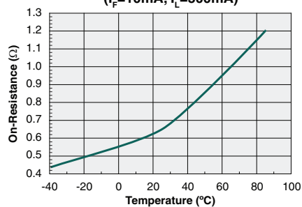
Typical On-Resistance vs. Temperature ( I_F=10\text{mA} , I_L=500\text{mA} )
