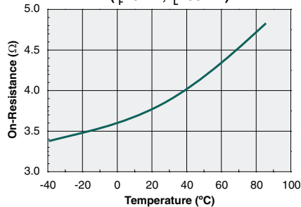
Typical On-Resistance vs. Temperature ( I_F=0\text{mA} , I_L=50\text{mA} )
