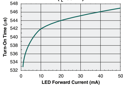
Typical Turn-On Time vs. LED Forward Current ( I_L=50\text{mA} )
