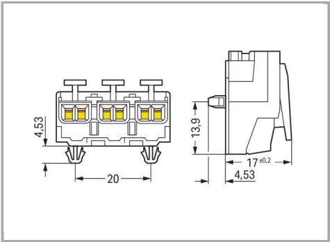
Snap-in foot
